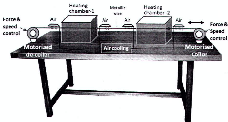
Figure 1 Schematic diagram of the proposed system for cyclic heat-treatment of metallic wires in the diameter range 0.3-0.5 mm
