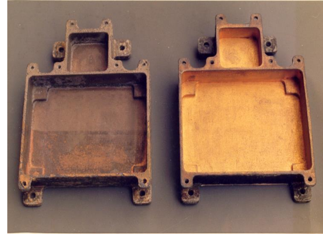
GOLD PLATING ON MAGNESIUM ALLOY BOXES
