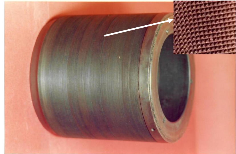
CHEMICAL MILLING OF SPAR TUBE (1/6 th MODEL)
