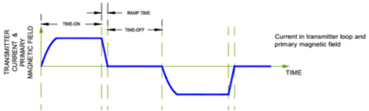
Figure 4.3: Typical Current pulse given to the transmittor coil
