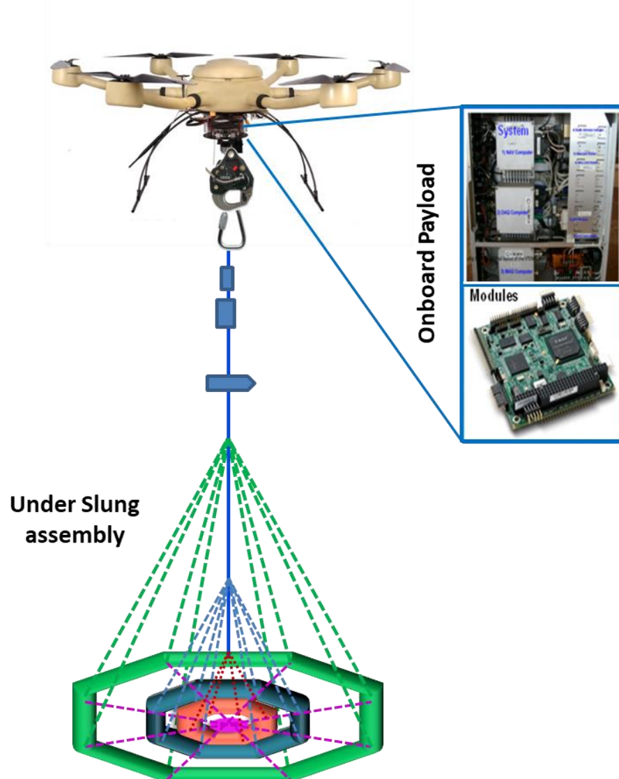
Figure 4.1: Schematic representation of the Field operations
