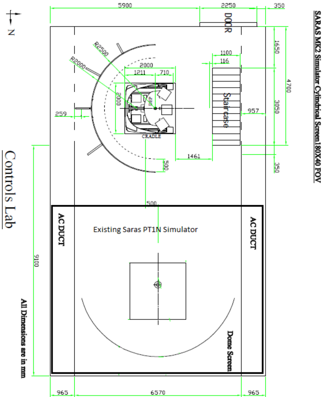
Drawing of mezzanine floor showing Proposed Saras Mk2 Simulator
