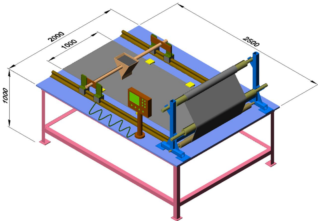
Fig. 1. Conceptual sketch of the feeder with dispenser machine
