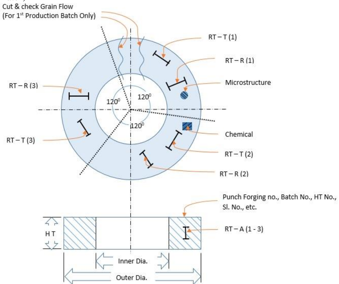
Figure-1: Test Specimen Location (On Rolled Ring / Ring Cut Segment / 1/Raw Material(RM) Melt Batch)
