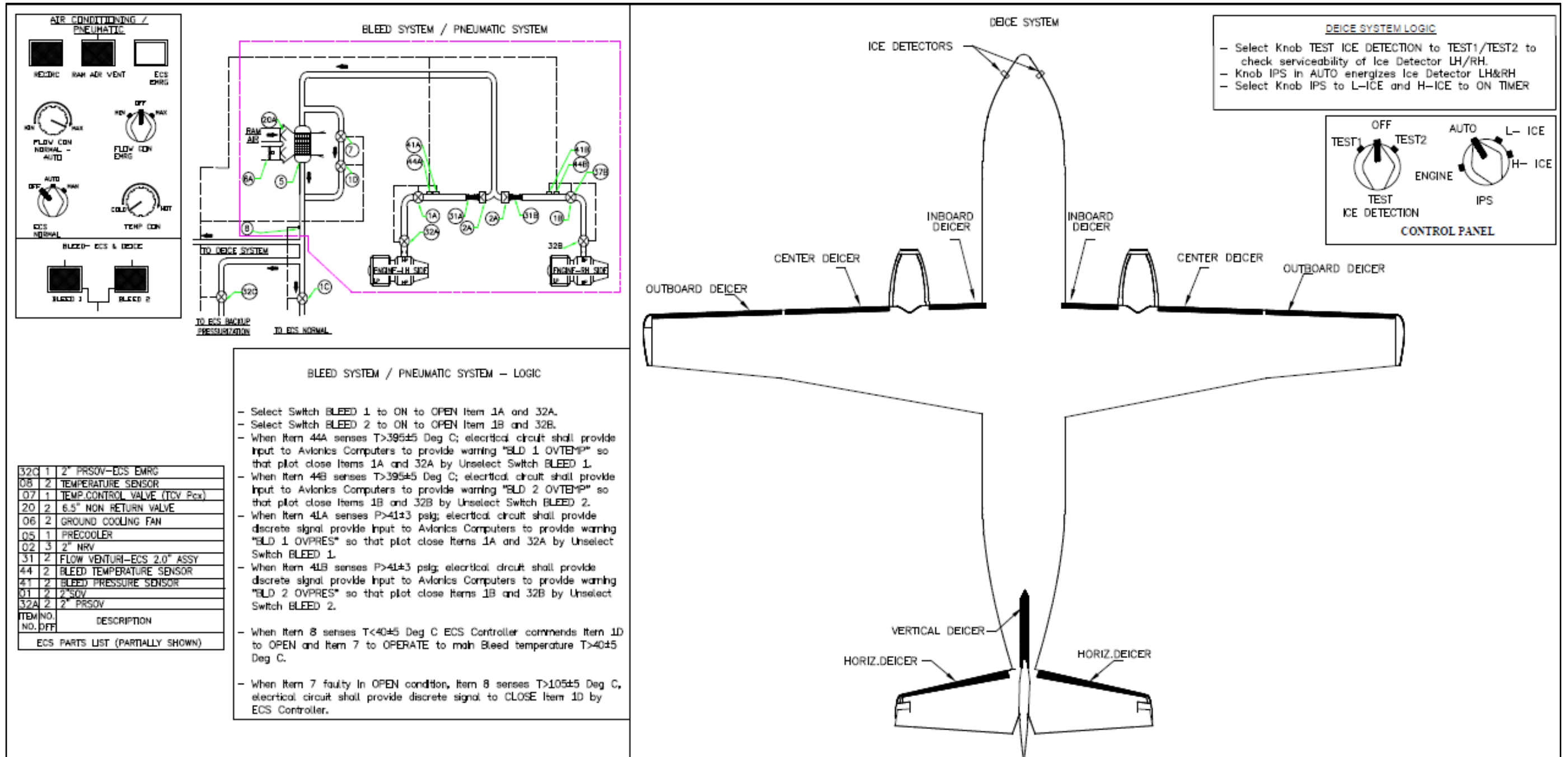
Figure 1: Saras Mk II Aircraft with Pneumatic Deicers - Leading Edges of Wing, VT and HT
