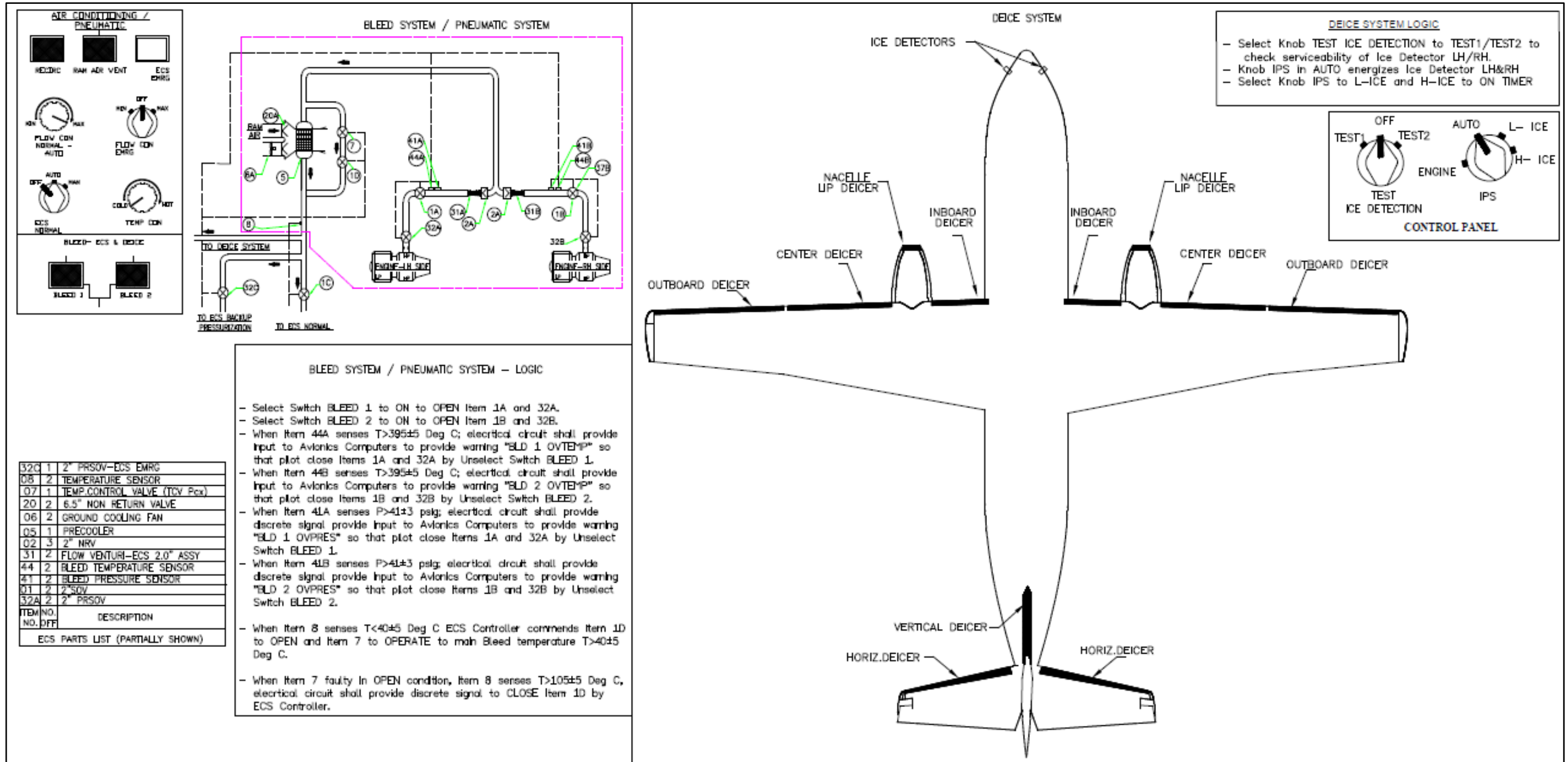
Figure 1: Saras Mk II Aircraft with Pneumatic Deicers - Leading Edges of Wing, VT, HT and Engine Air Intake Lip
